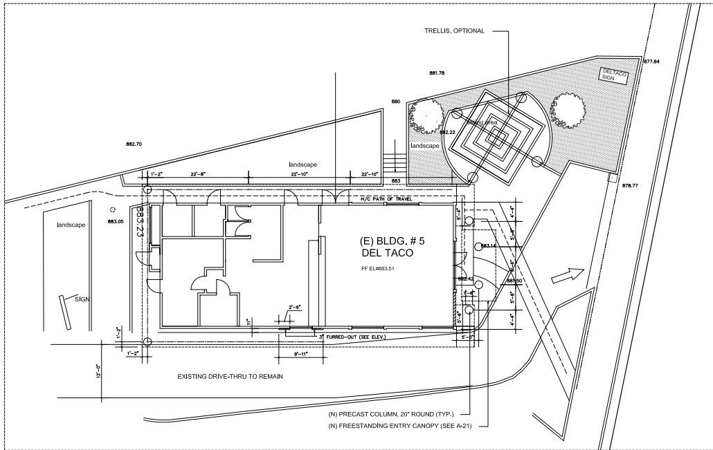
IMPROVED FLOOR PLAN SCALE: 1/8"=1'-0"
