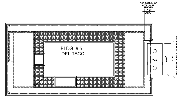
IMPROVED ROOF PLAN SCALE: 1/8"=1'-0"
